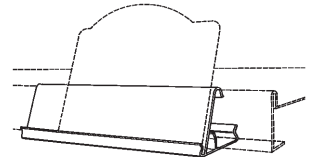
HCO: Clip-On Holder adapted to mezzanine shelf.
